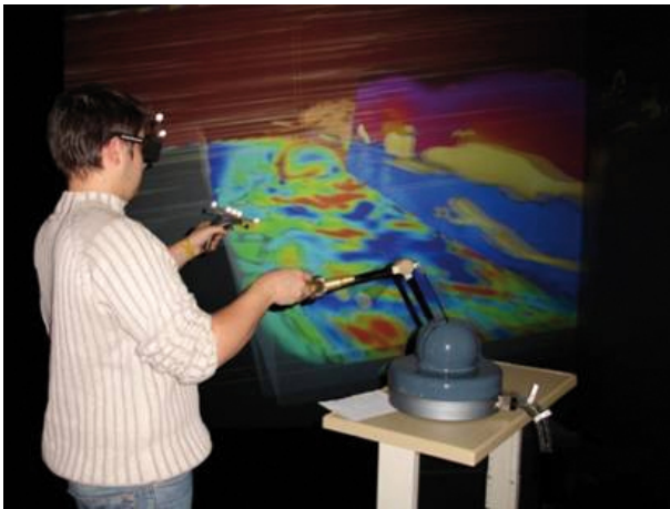
Figure 1: An accurate positioning of a colored cutting plane, in the CFD immersive application of the ANR "CoRSAIRE" project.
